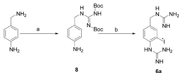
Scheme 3. Reagents: (a) N,N' -Bis- tert -butoxycarbonylthiourea, Triethylamine, Mukaiyama reagent; (b) (i) Radioiodine, NCS (ii) cyanamide; (iii) Trifluoroacetic acid/water/triisopropylsilane (95/2.5/2.5).
