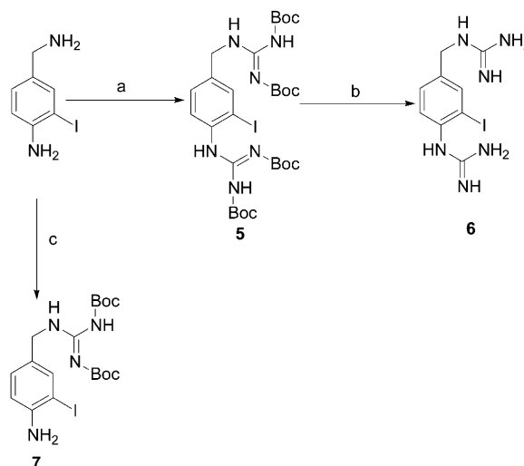
Scheme 2. Reagents: (a) N,N' -Bis- tert -butoxycarbonylthiourea, Triethylamine, Mukaiyama reagent; (b) Trifluoroacetic acid/water/triisopropylsilane. (95/2.5/2.5); (c) N,N' -Bis- tert -butoxycarbonyl-S-methylisothiourea, Triethylamine, DMF.
