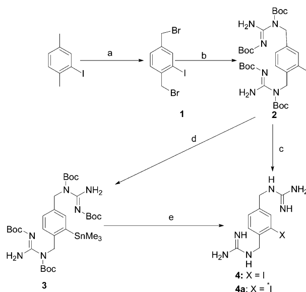
Scheme 1. Reagents: (a) N -Bromosuccinimide, 1,1'-Azobis-(cyclohexanecarbonitrile), DCE; (b) N,N' -bis- tert -butoxycarbonylguanidine, NaH, DMF; (c) Trifluoroacetic acid/water/triisopropylsilane (95/2.5/2.5), methylene chloride; (d) Hexamethyditin, Bis-(triphenylphosphine) palladium dichloride, dioxane; (e) i -Radioiodine, NCS ii-c.
